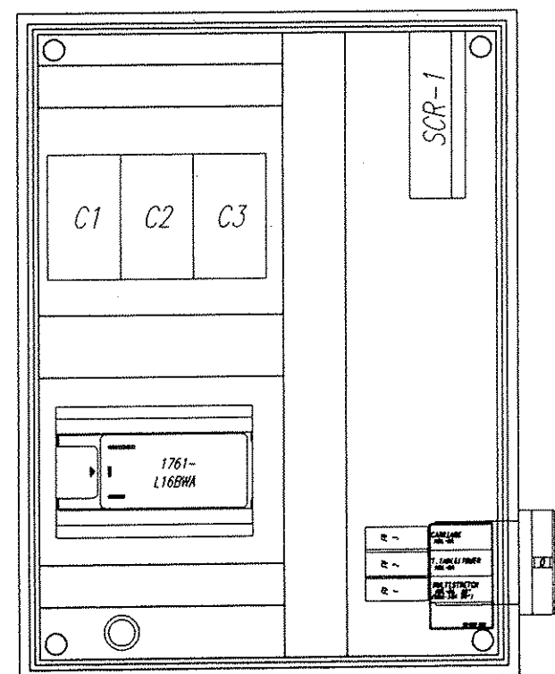
M67-10 PANEL LAYOUT 16 x 12 x 06
