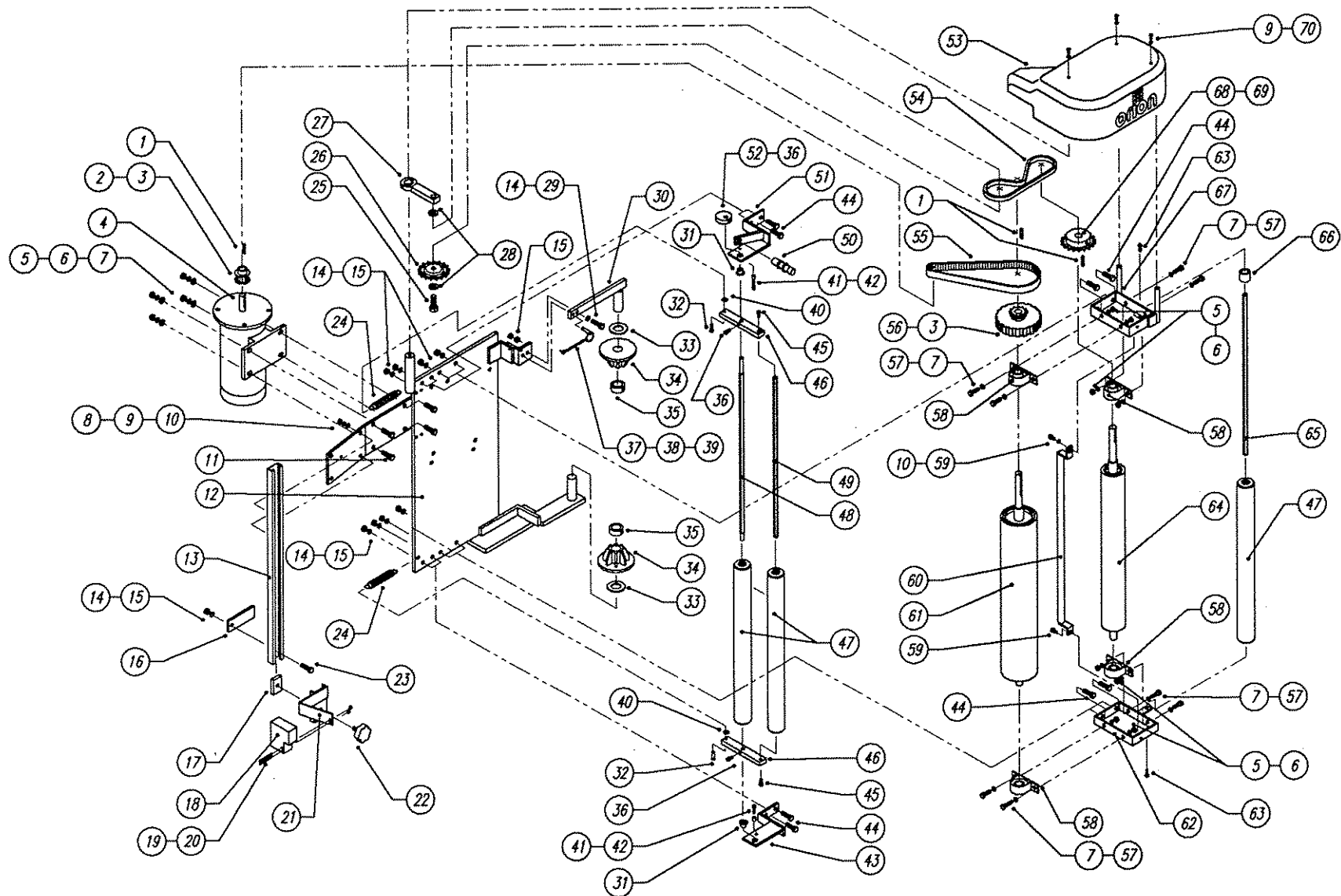
20" FILM CARRIAGE FOR STD MONGOOSE PART # 405102 - ASS'Y
