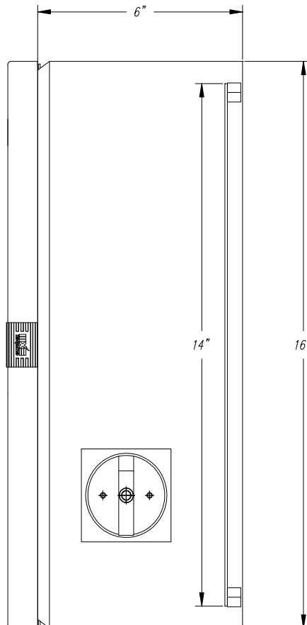
HL77-16306 PANEL LAYOUT PANEL STICKER PN-500 104 (5412 ESCH161206)
