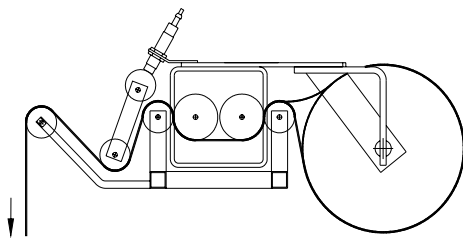
Fig. 2 CLOSED CRADLE
