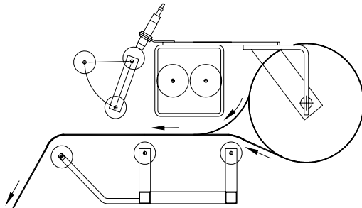
Fig. 1 OPEN CRADLE
