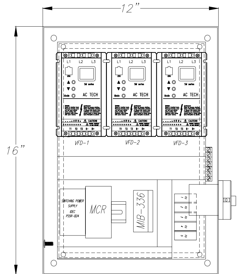
BACK PLATE
