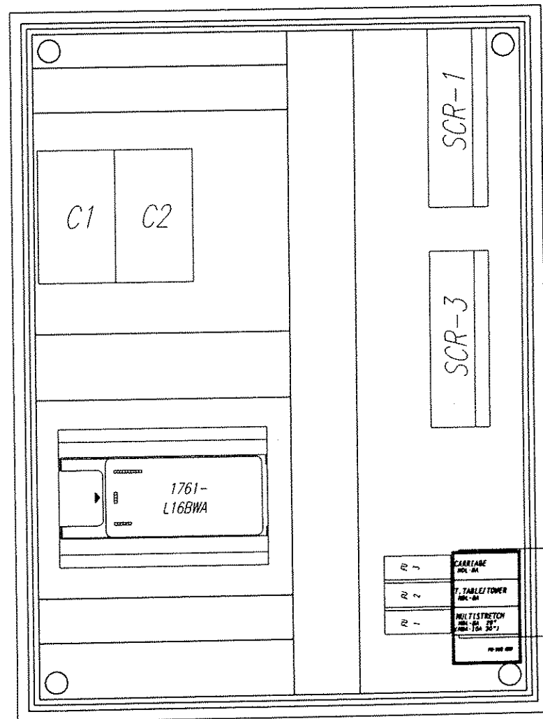
HL55-10 PANEL LAYOUT
